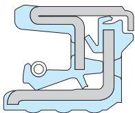
Simmerring® Cassette seal type 2
